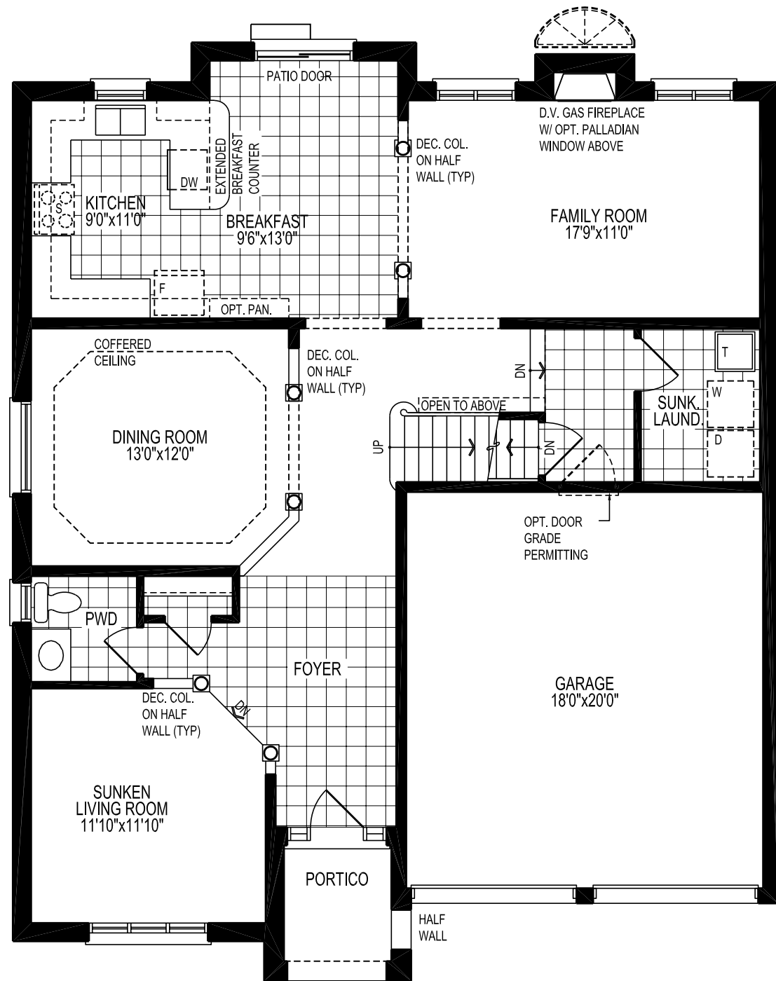
GROUND FLOOR PLAN 'A'
