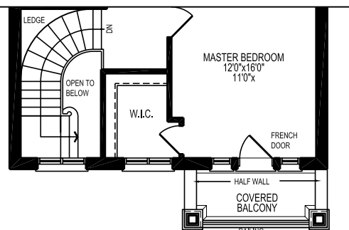
SECOND FLOOR PLAN 'A'
