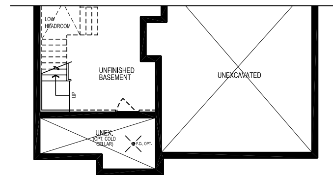
PARTIAL BASEMENT PLAN 'B'
