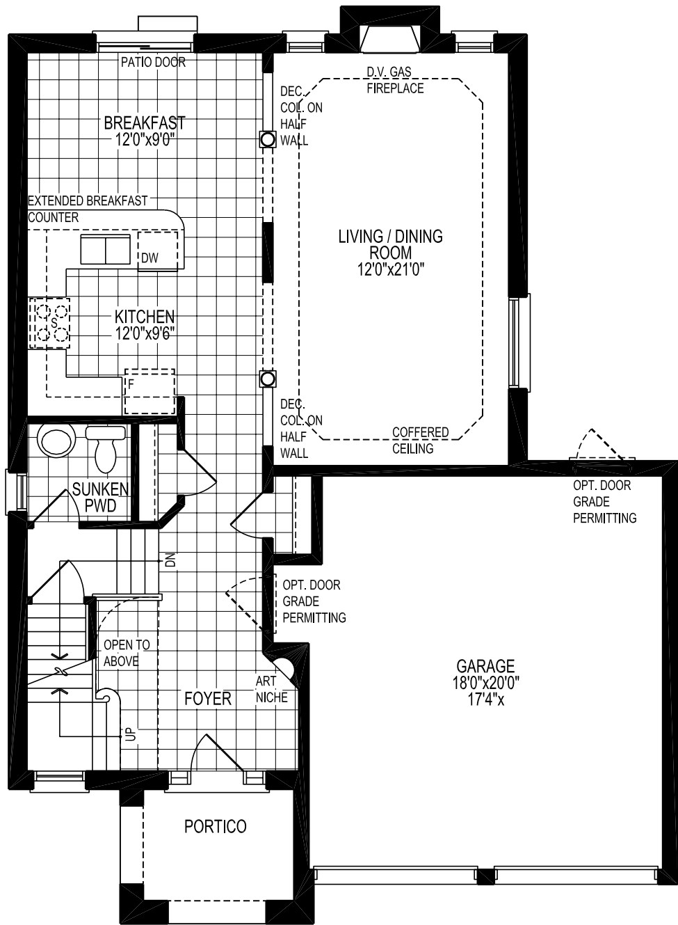
GROUND FLOOR PLAN 'A' & 'C'
